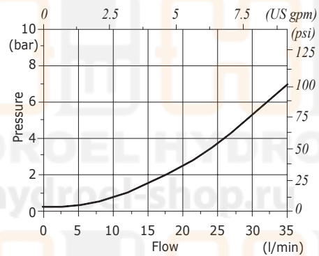
VRFU9003 pressure drop vs. flow (B→A)
